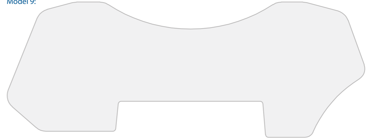
Model 9:
