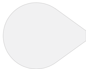
Model 7
