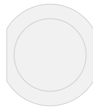
Model 3:
