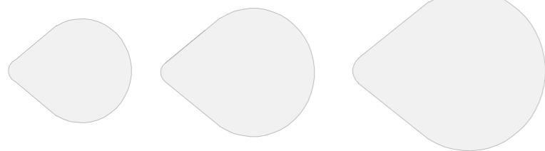
Model 5:
