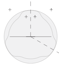
Model 4:
